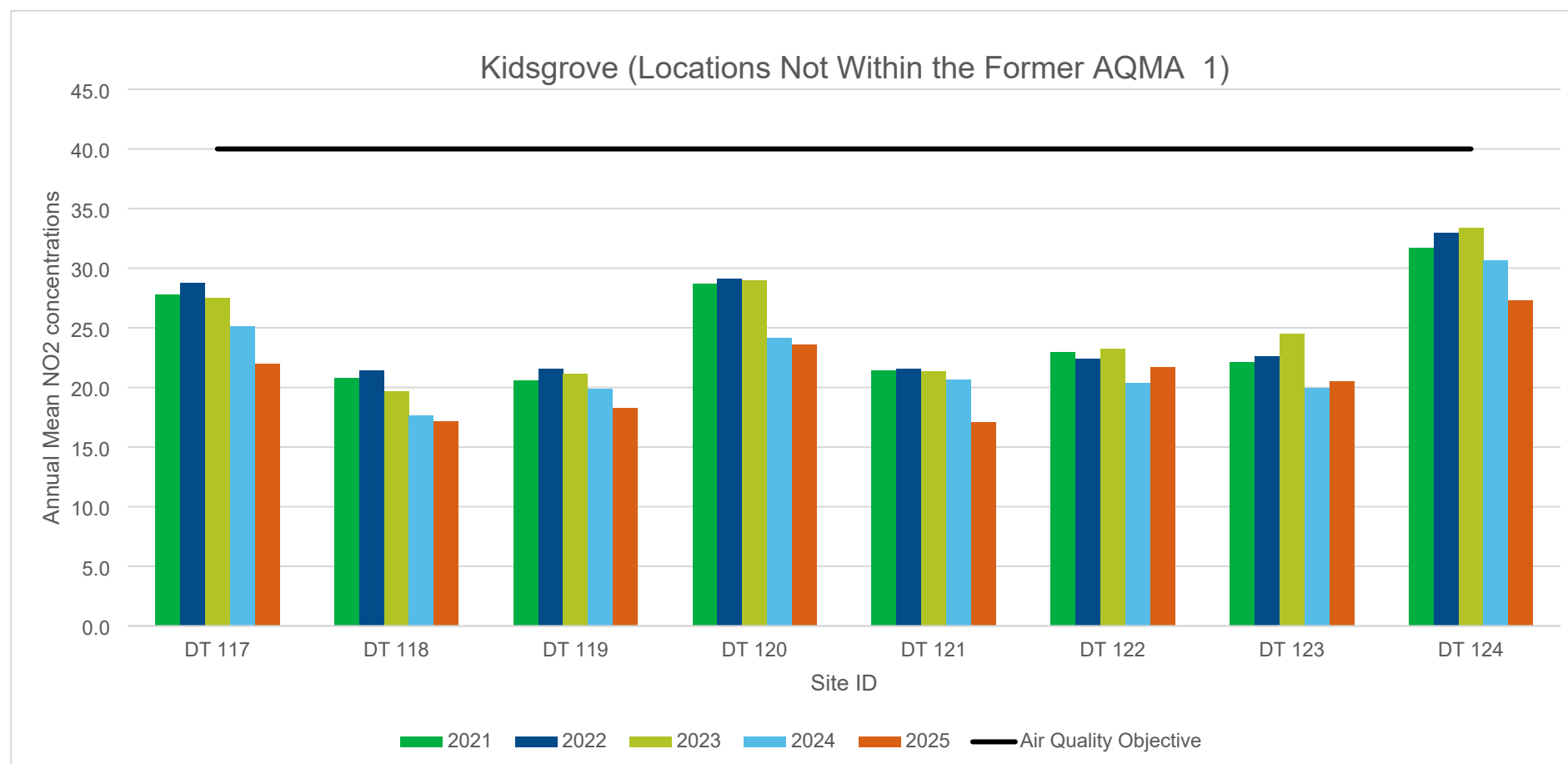
Figure A-4) Trends in annual mean NO 2 concentrations 2021 to 2025 – Kidsgrove East and West (outside the Former AQMA 1)
