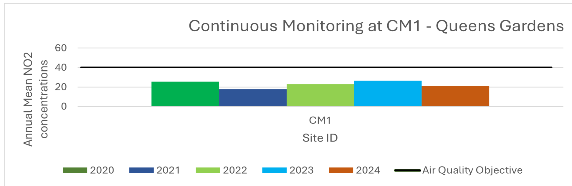
Figure A-0) Trends in annual mean NO 2 concentrations 2020 to 2024 – Continuous Monitoring Station (Queens Gardens) (Within AQMA 2).
